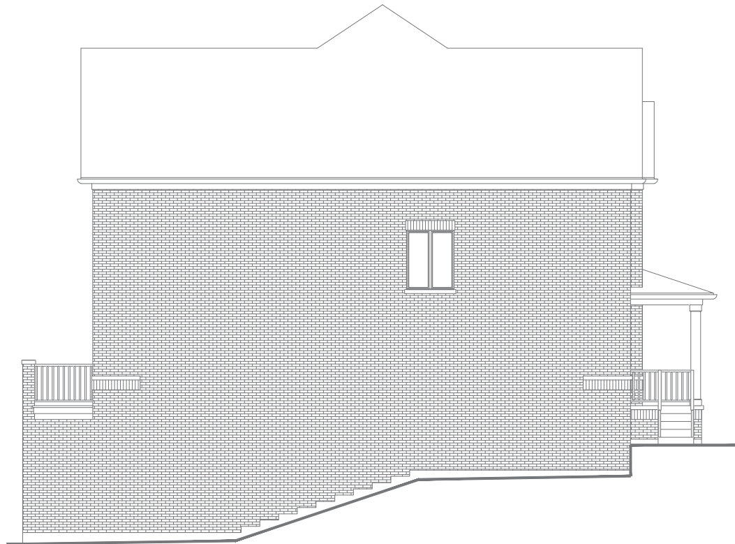
LEFT SIDE ELEVATION 'A2' INTERIOR END
