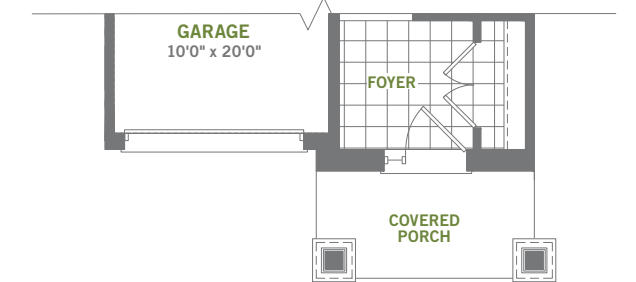
PARTIAL GROUND FLOOR 'B1'
