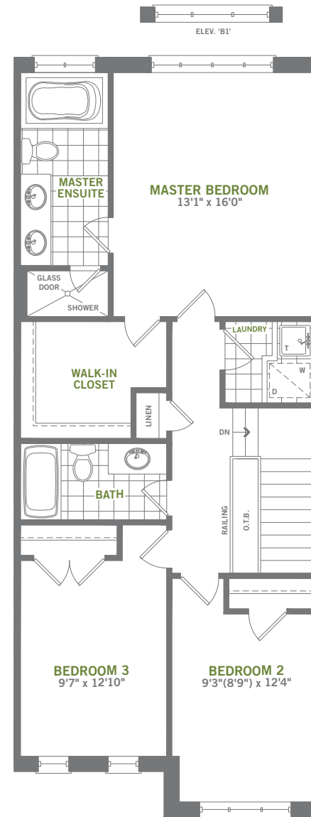
SECOND FLOOR 'A1'
