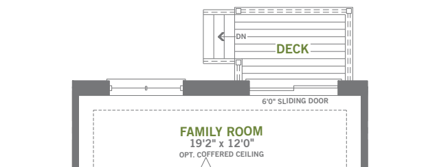
PARTIAL GROUND FLOOR 'B1' LOB CONDITION
