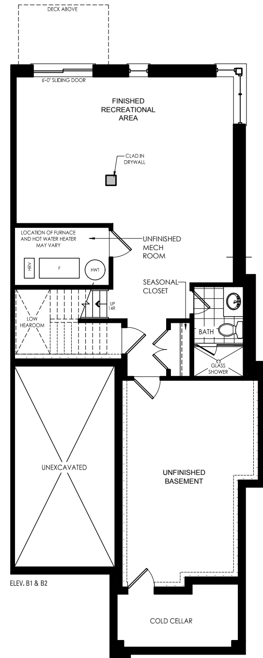
walkout basement
