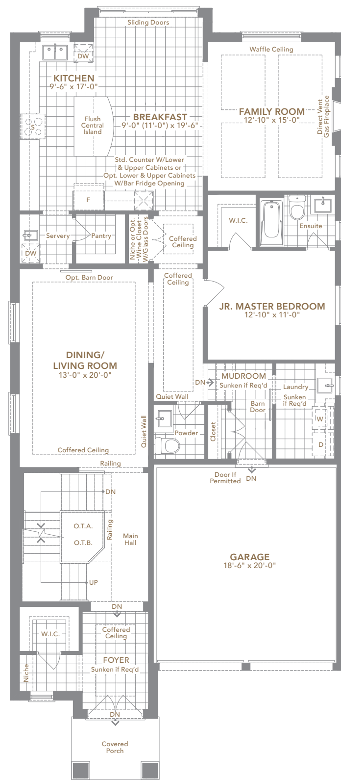
ELEVATION A ALTERNATE MAIN FLOOR (JR. MASTER BEDROOM)
