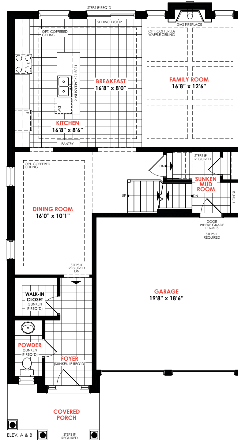
Main Floor
