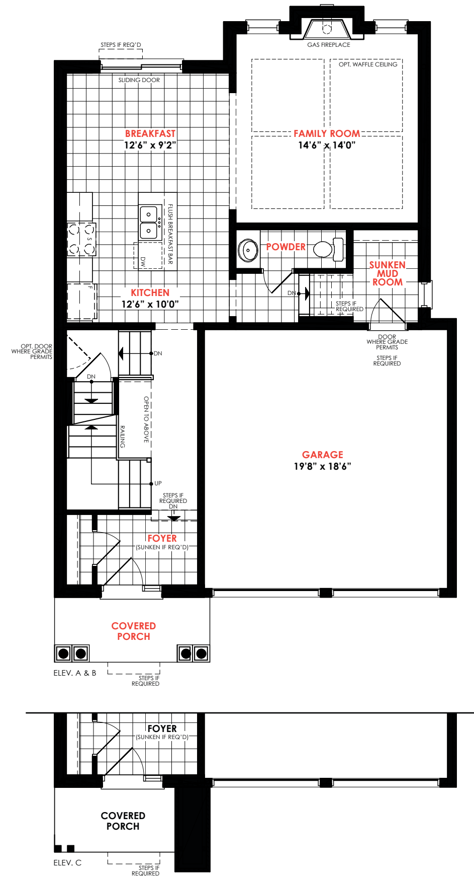
Main Floor
