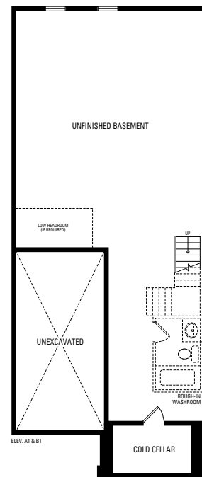
BASEMENT
